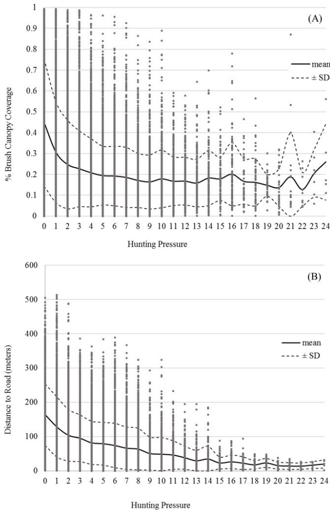
Fig. 4. A) Percent brush canopy cover and B) distance to road per 50-meter x 50-meter grid cell, categorized by total hunting effort from quail hunts recorded during the 2018–2019, 2019–2020, and 2020–2021 hunting seasons in Jim Hogg County, Texas, USA.
